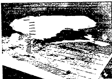
A computer model representation of a blizzard over the Colorado Front Range area, produced jointly by NOAA's Forecast Systems Laboratory (FSL) and the Colorado State University. The image represents a six hour forecast, looking over Colorado from the southeast. The white/gray area depicts the forecast region for significant clouds, and the red area within the clouds represents the region in which aircraft icing is likely to occur.
