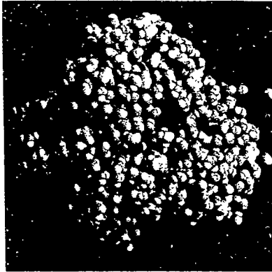
The myoglobin protein with a hydration of 350 water molecules.
