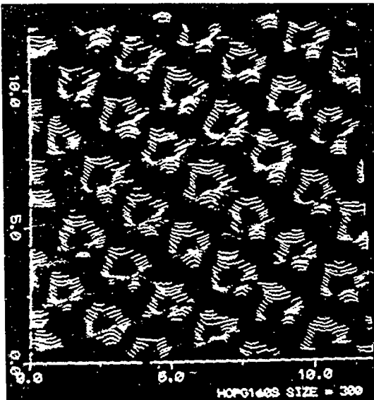
In this closeup of the sample on the preceding page, atomic-level structures of carbon rings at the surface are seen. A button permits energy to be supplied on demand through the STM tip to modify the surface by breaking bonds, displacing various structures and enabling physical and chemical reactions.
