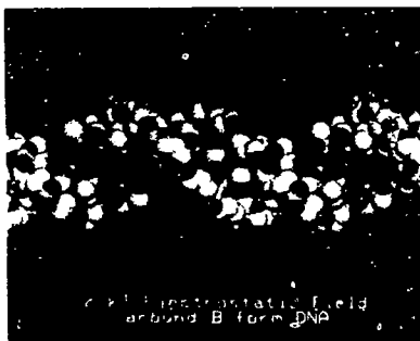
Calculation of the binding of small molecules to DNA and other biological macromolecules depends upon a complex interaction of electrostatic fields, solvent-accessible surface, and other physicochemical properties. Structure-based drug design is a key biomedical HPCC Grand Challenge.
