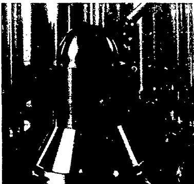
A computer-controlled coordinate measuring machine determines the exact dimensions of a precision-machined stainless steel part. NIST researchers use this and similar instruments to devise ways to improve machine tool performance.
