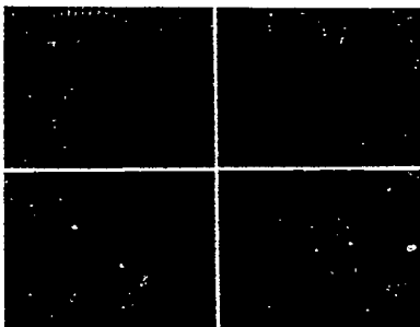
Researchers evaluate molecular properties of carcinogens from pollution sources. The image shows electric field vectors for benzopyrene.
